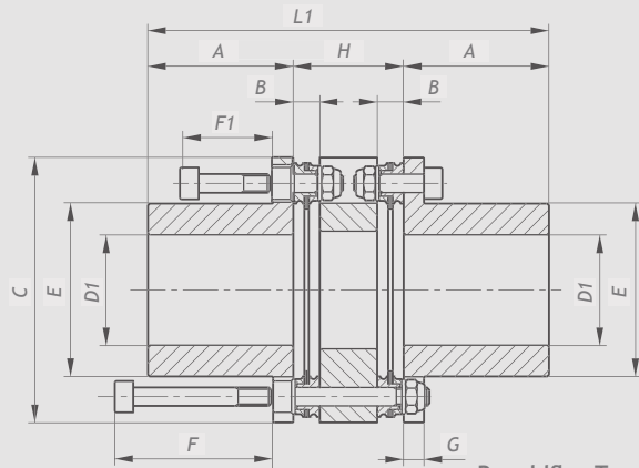
Renoldflex Type B H-MIN
