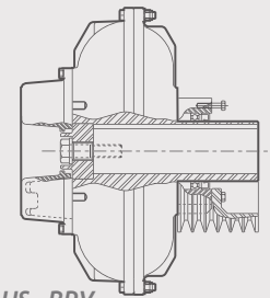
Type: HS..RPV
