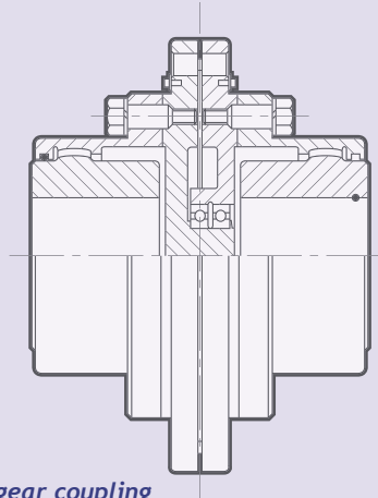
Shear pin gear coupling
