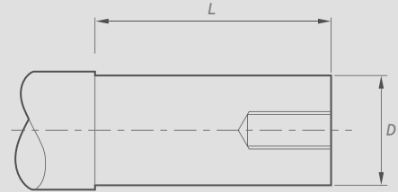
Motor shaft details
