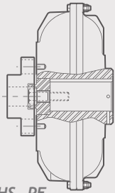
Type: HS..PF
