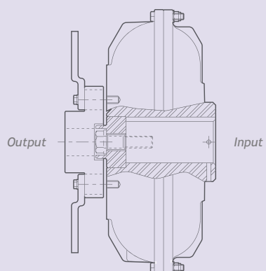
Hydrastart Pinflex Coupling and brake disc
