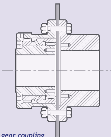
Disk brake gear coupling
