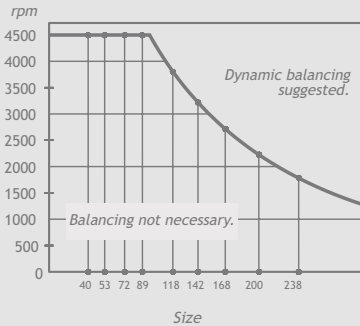
[ fig 05 ] Balancing
