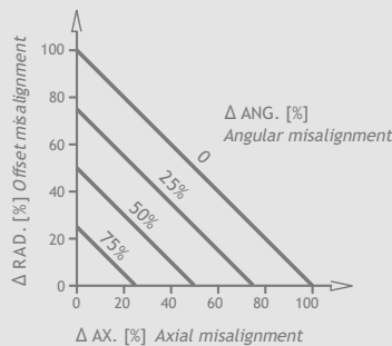
[ fig 02 ] Misalignment diagram
