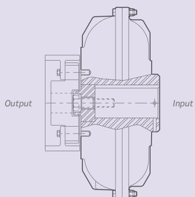
Hydrastart Pinflex Coupling and brake drum
