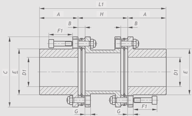
Renoldflex Type B
