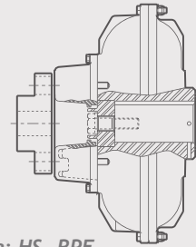
Type: HS..RPF
