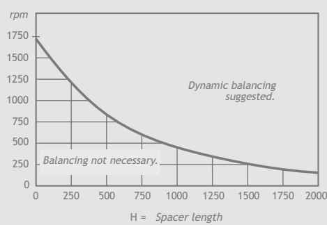
[ fig 06 ] Balancing
