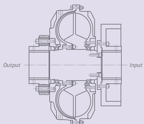
Hydrastart Pinflex/Rigid Coupling and brake drum/disc
