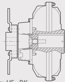
Type: HS..RK
