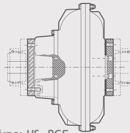
Type: HS..RGF
