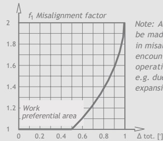
[ fig 03 ] Misalignment factor f_1
