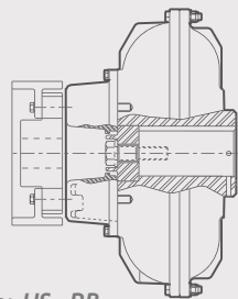
Type: HS..RB
